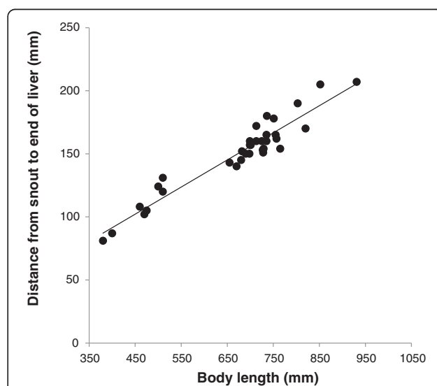
Figure 1 Relationship between distance from the snout to the end of the liver ( L_{EL} ) and total body length ( L_T ). The line shows the linear regression model ( n = 34 ).
