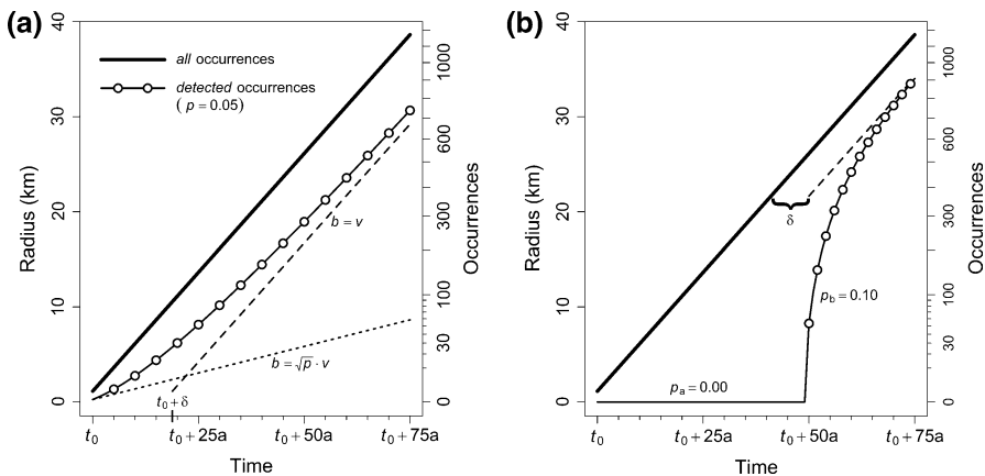
Fig. 1 Trajectories of expansion and detection of an invading species according to the model proposed in the text, illustrated for the case of a constant expansion speed v=500 m/a. In this situation, the radius r of the total AOO increases linearly (all occurrences, bold lines), whereas the radius \rho of the known AOO lags behind (cumulative detected occurrences, thin solid lines). The dotted line (a) shows the initial slope b of the detection curve; the broken lines show the asymptotes that are approached by the detection curves. The ‘detection debt’ \delta is the time by which the asymptote is displaced from the expansion trajectory. The slopes of the true expansion trajectory and of the asymptote equal the expansion speed ( b=v ). The detection rate p is constant at 5% in (a), whereas it changes after 50 years from 0 to 10% in (b). Note that the right y-axes are on square-root scale (e.g. a radius r of 20 km corresponds to an AOO of \pi r^2 = 1256 km 2 , and thus to 314 occurrences or grid occupancies of 4 km 2 each)
