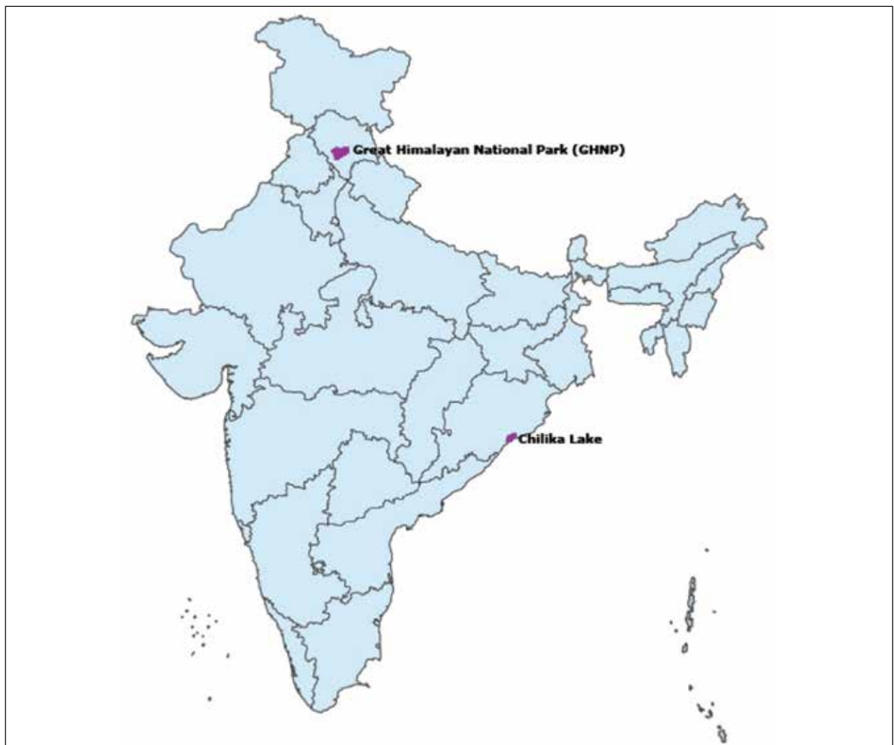
Figure 1: Location of two pilot sites
