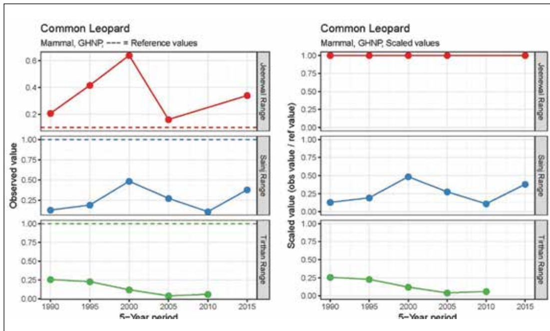
Figure 49: Observed and scaled value of Common Leopard
