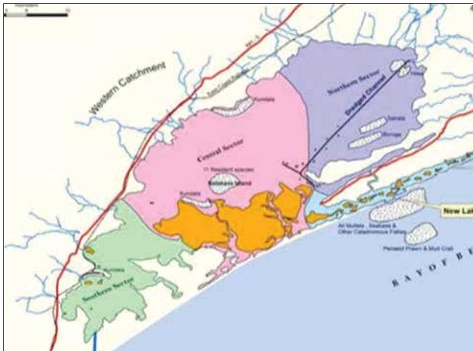
Figure 2: Chilika Lake and the demarcated sectors
