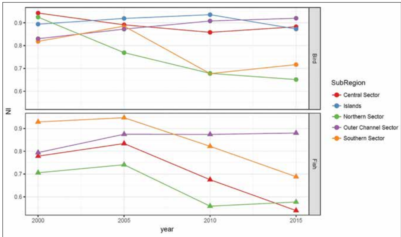
Figure 9: Thematic NI value (5-year periods) for the five areas of Chilika Lake
