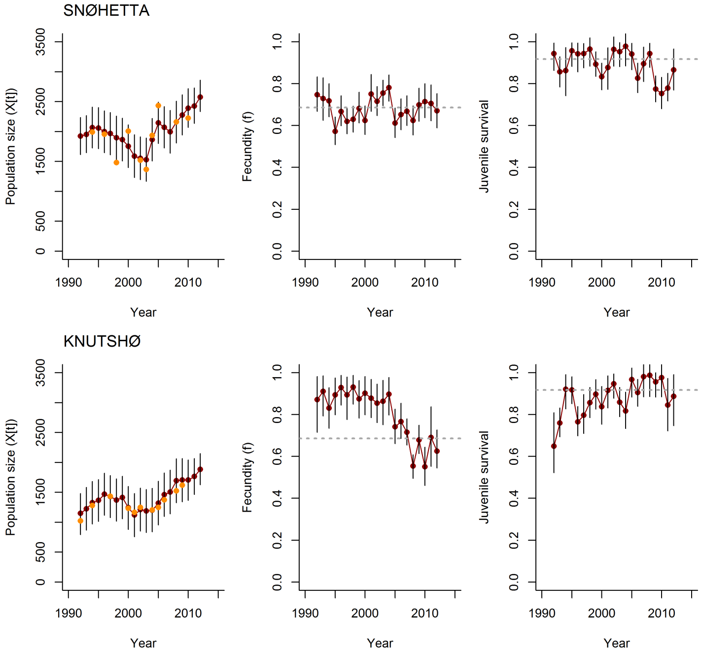
Fig 5. Estimated population trajectories. Estimated time series of abundance (left panels), fecundity ( f ) (middle panels) and juvenile summer survival probability ( \phi_1 ) (right panels) for Snøhetta (upper panels) and Knutshø (bottom panels) respectively. Model output is based on M1 (see Methods section).
